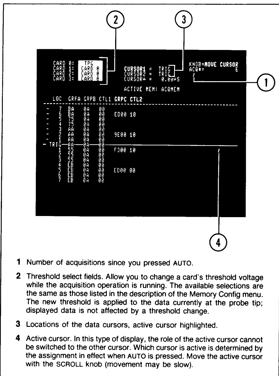
Figure 4-9. Status display for COMPARE ACOMEM TO REFMEM, DISPLAY AND REACQUIRE action. The bottom half of the display is shown in State Table or Timing Diagram format, depending on which data display format was last used. Moving the cursor affects the comparison limits if BETWEEN CURSORS is selected.
