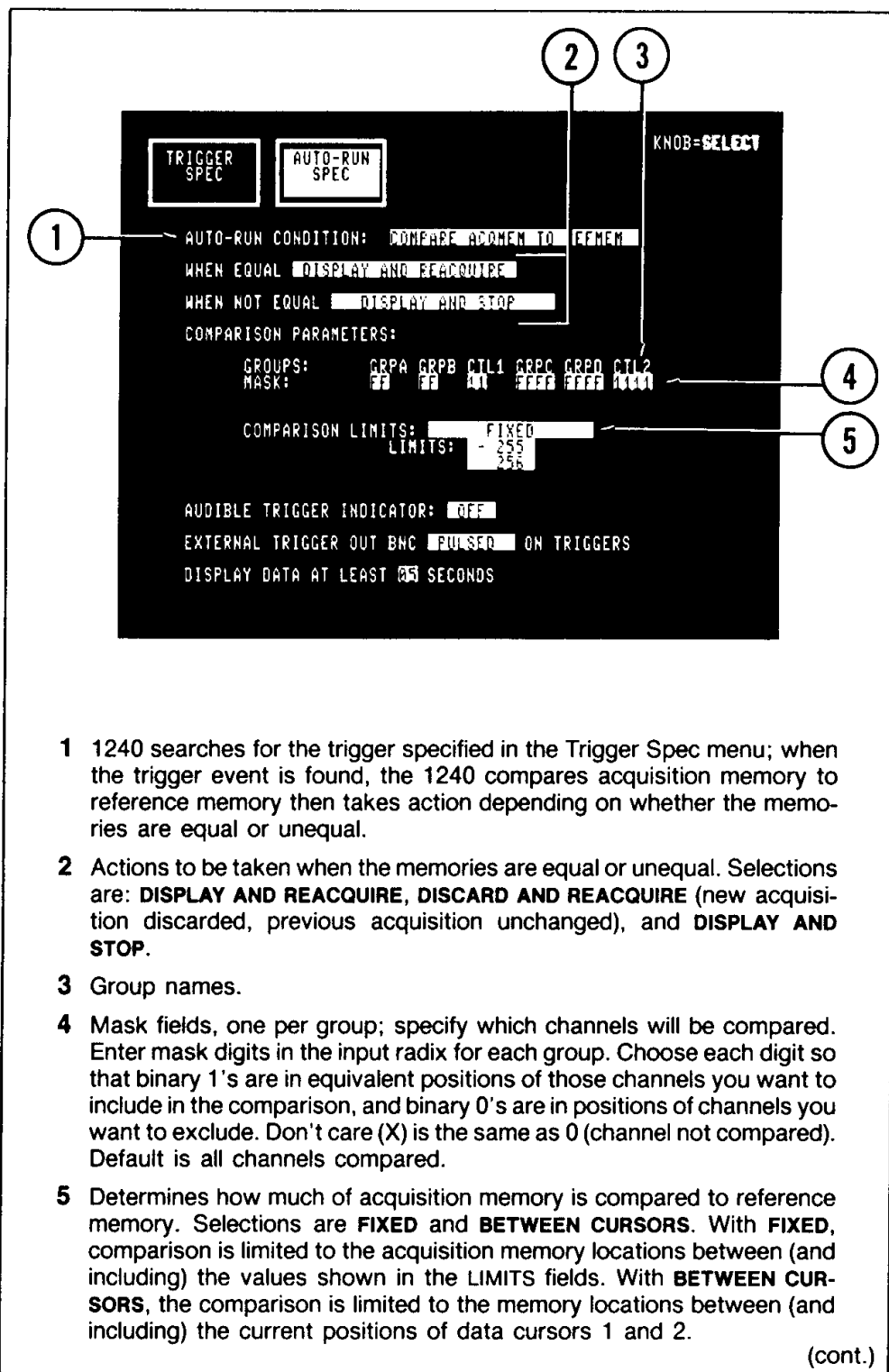
Figure 4-6. Menu display for the COMPARE ACQMEM TO REFMEM Auto-Run condition. The selected data in acquisition memory must be identical to the corresponding data in reference memory, including time relationships between two-timebase data, for the memories to be considered equal.
