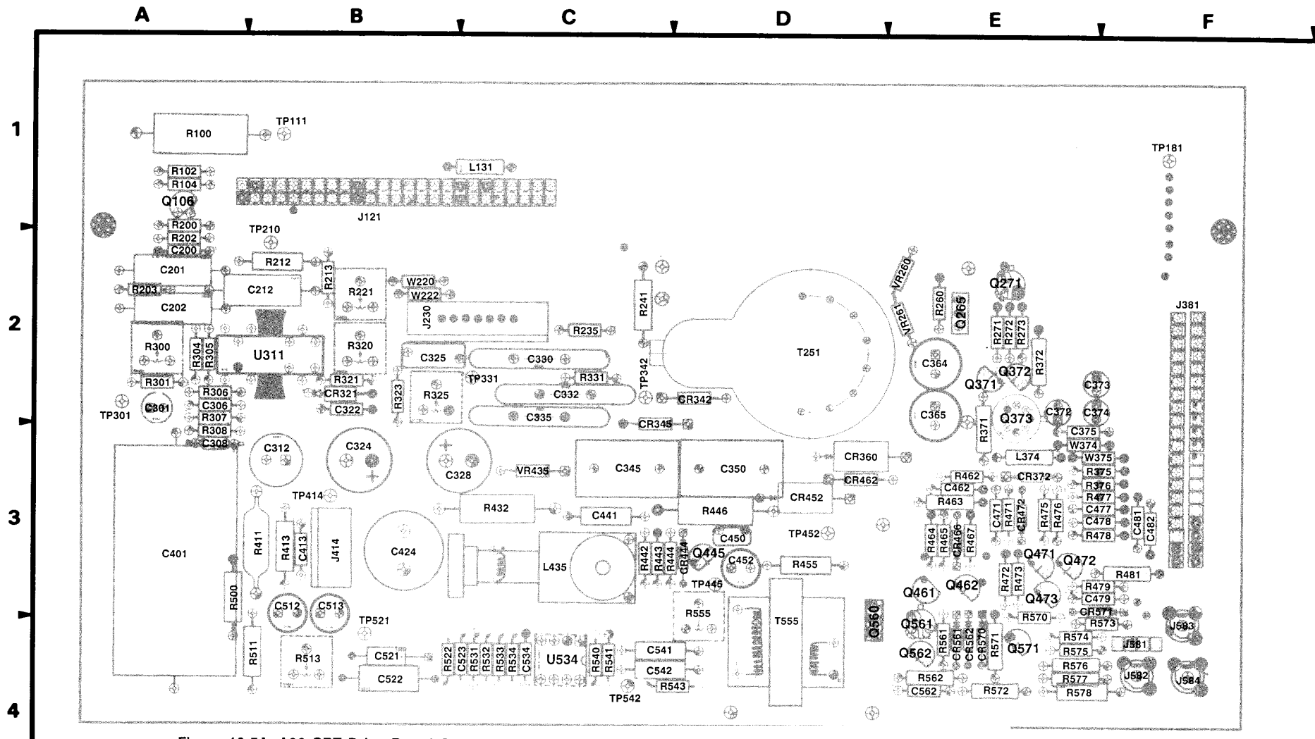
Figure 10-5A. A06 CRT Drive Board Component Locations (R090000 & below)
