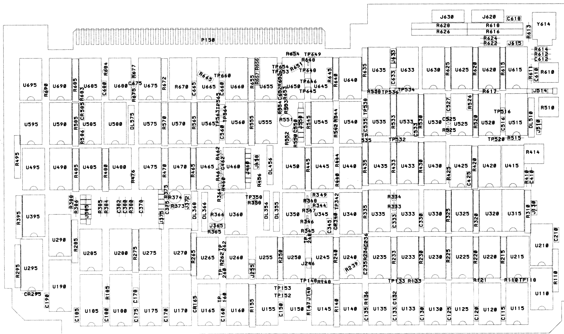
Figure 10-17a. A14 Trigger Board Component Locations (670-7523-09 & below).
