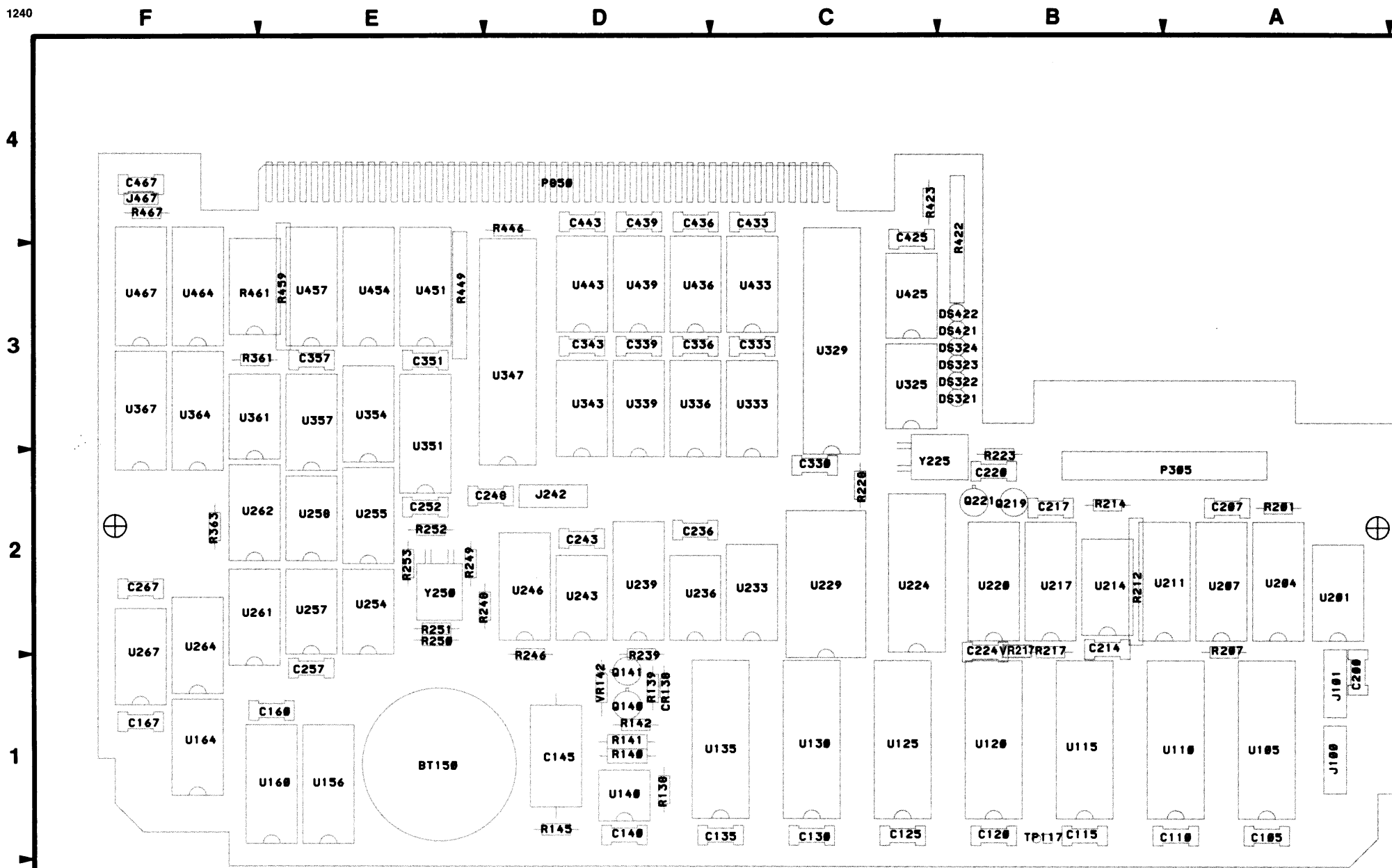
Figure 10-11. A09 Control Processor Board Component Locations.
