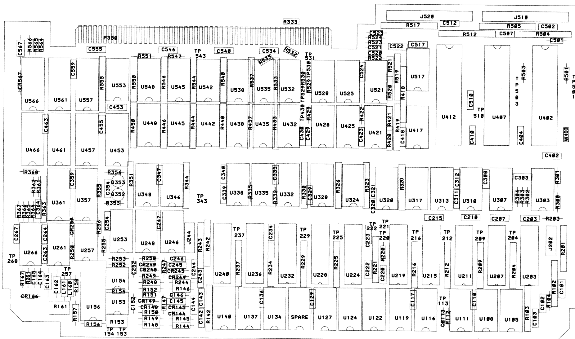
Figure 10-21. A16 18-Channel Acquisition Board Component Locations.
