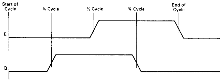
Figure 11 HD6809E Clock Generator
