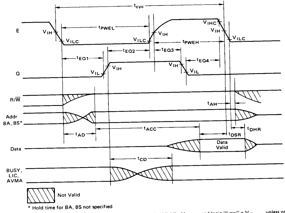
(NOTE) Waveform measurements for all inputs and outputs are specified at logic "High" = V_{IHmin} and logic "Low" = V_{ILmax} unless otherwise specified. Figure 1 Read Data from Memory or Peripherals
