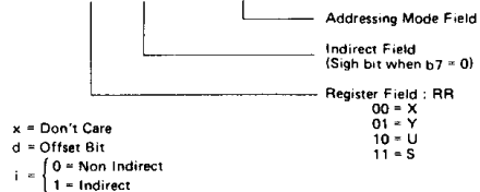
Figure 16 Index Addressing Postbyte Register Bit Assignments
