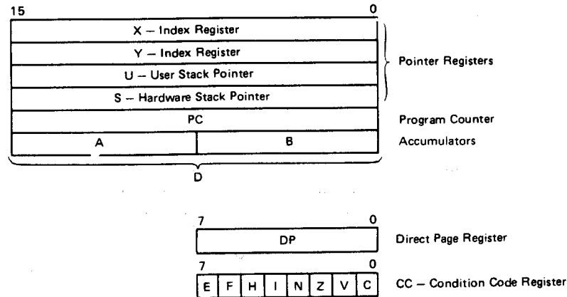
Figure 5 Programming Model of The Microprocessing Unit
