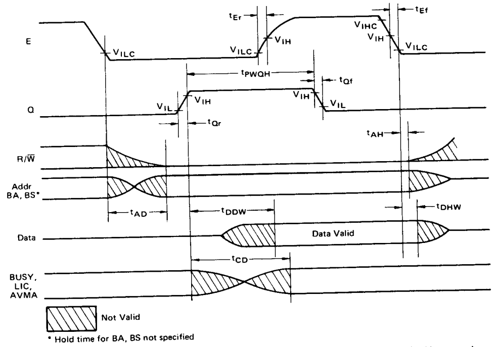
(NOTE) Waveform measurements for all inputs and outputs are specified at logic "High" = V_{IHmin} and logic "Low" = V_{ILmax} unless otherwise specified. Figure 2 Write Data to Memory or Peripherals
